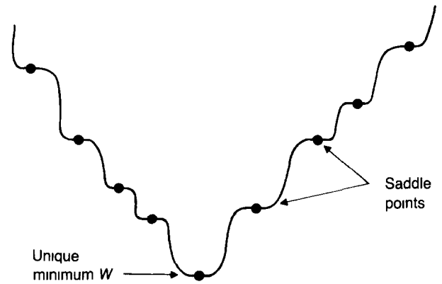
FIGURE 2. The landscape of E .
